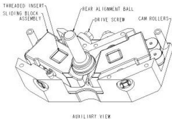
Figure 6. Shutter Insert Adjustment Mechanism
