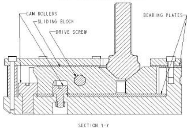
Figure 6. Shutter Insert Adjustment Mechanism
