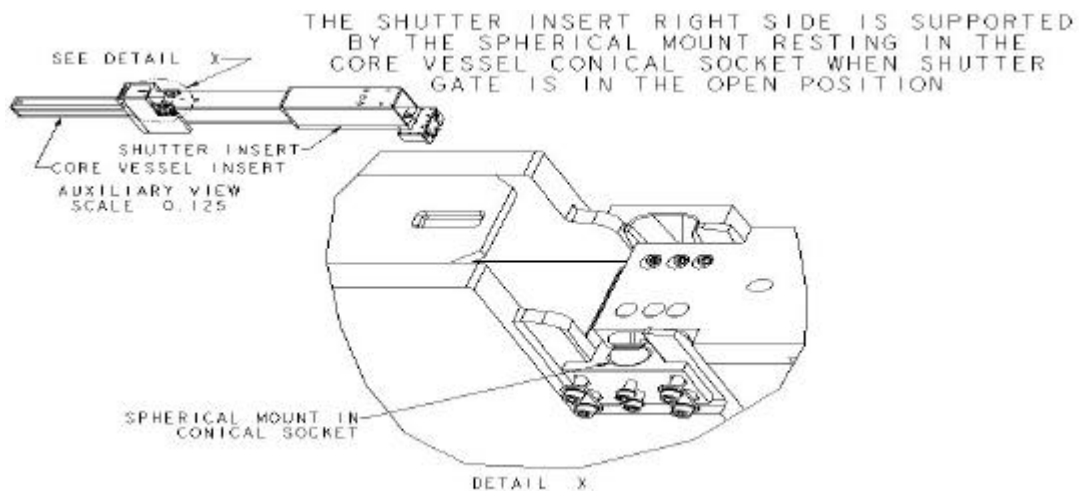
Figure 3. DVTS Shutter Insert Right Alignment Support
