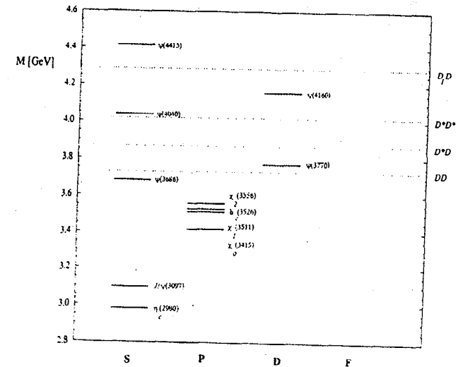
Fig. 3: The 11 known c\bar{c} states. All have J^{PC} = 1^{--} except the 1P multiplet near 3.5 GeV and the J^{PC} = 0^{-+} \eta_c(2980) . Some open charm thresholds are also shown.
