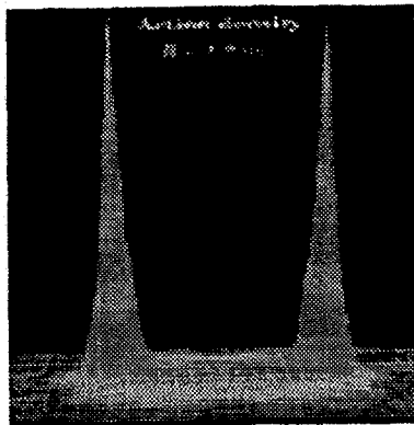
Fig. 1: The gluonic flux tube between static quark sources (Bali et al. [1]).
