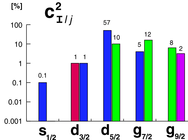
Fig. 1. Structure of the 3/2^+[411] ^{131}\text{Eu} ground-state as composed of the spherical lj orbitals s_{1/2} , d_{3/2} , d_{5/2} , g_{7/2} and g_{9/2} . The fractions of the wave function coupled to the final I=0^+ (red), 2^+ (blue), 4^+ (green) and 6^+ (violet) states in ^{130}\text{Sm} via proton emission are indicated.
