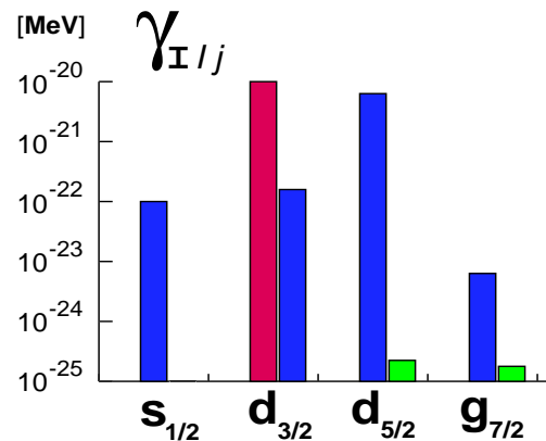
Fig. 2. Main components of the decay width (in MeV) for the proton transitions from the ^{131}\text{Eu} ground-state to the I=0^+ ground state (red) and to the excited I=2^+ (blue) and I=4^+ (green) states of ^{130}\text{Sm} .
