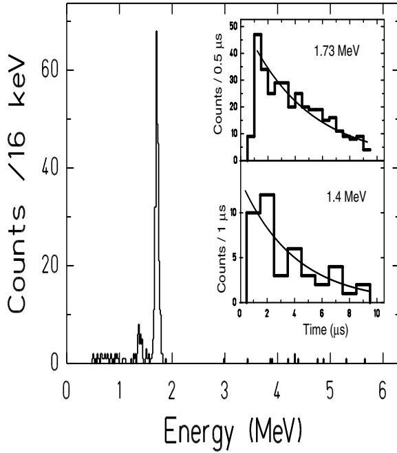
Fig. 3. An energy spectrum and decay patterns of proton lines originating from ^{145}\text{Tm} radioactivity.
