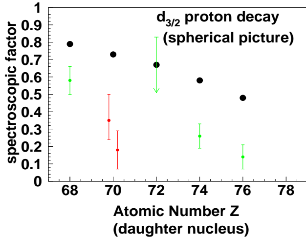
Fig. 4. Spectroscopic factors for the l = 2 proton emission analysed assuming spherical \pi d_{3/2} \otimes 0^+ parent state configuration. Red symbols denote recently observed decays of ^{150m}\text{Lu} and ^{151m}\text{Lu} . Black dots indicate the calculated vacancies u^2 for respective \pi d_{3/2} states.
