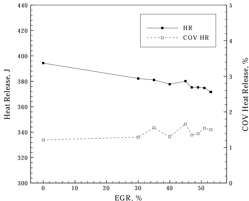
Figure 1. Heat release and COV showed no sudden changes as EGR level was increased.
