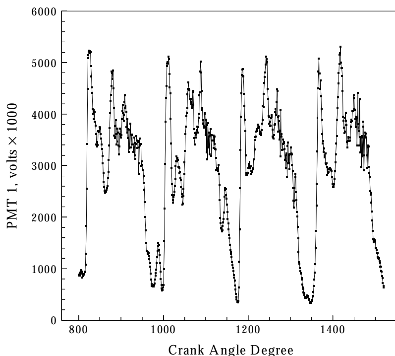
Figure 7. Example of the crank angle resolved signal from the DPS for a single engine cycle. Particulates from each cylinder event are clearly visible.
