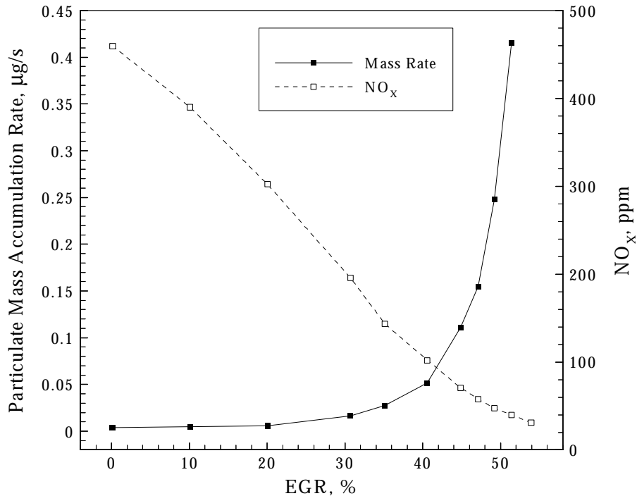
Figure 4. The intersection of the particulate mass accumulation rate and NO x curves represents a region where the engine out particulate mass and NO x concentration are minimized for this engine condition.
