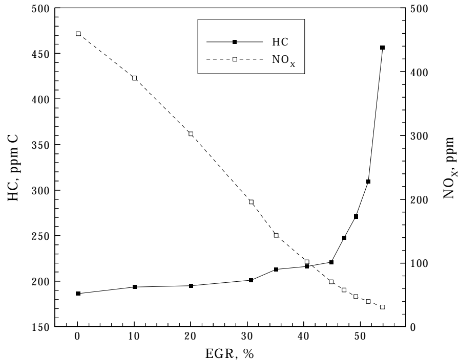
Figure 3. Trade-off between HC and NO x concentration as a function of EGR level.
