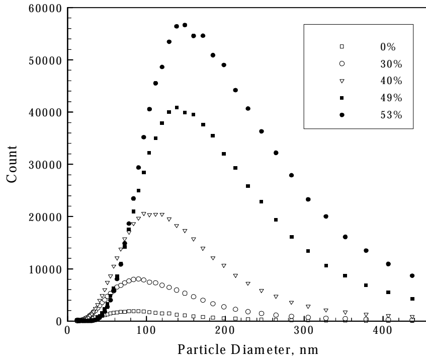
Figure 5. Time-averaged size distributions as measured by the SMPS. The overall number and size of particles increases with increasing EGR.
