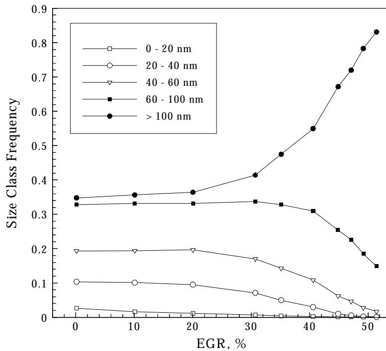
Figure 6. Frequency of occurrence of particle size classes as a function of EGR. Frequency of smaller particles decreases as the frequency of larger particles increases at higher EGR levels.
