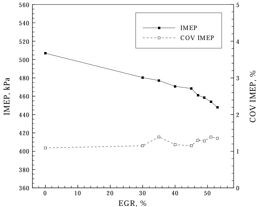
Figure 2. IMEP and COV showed no sudden changes as EGR level was increased.
