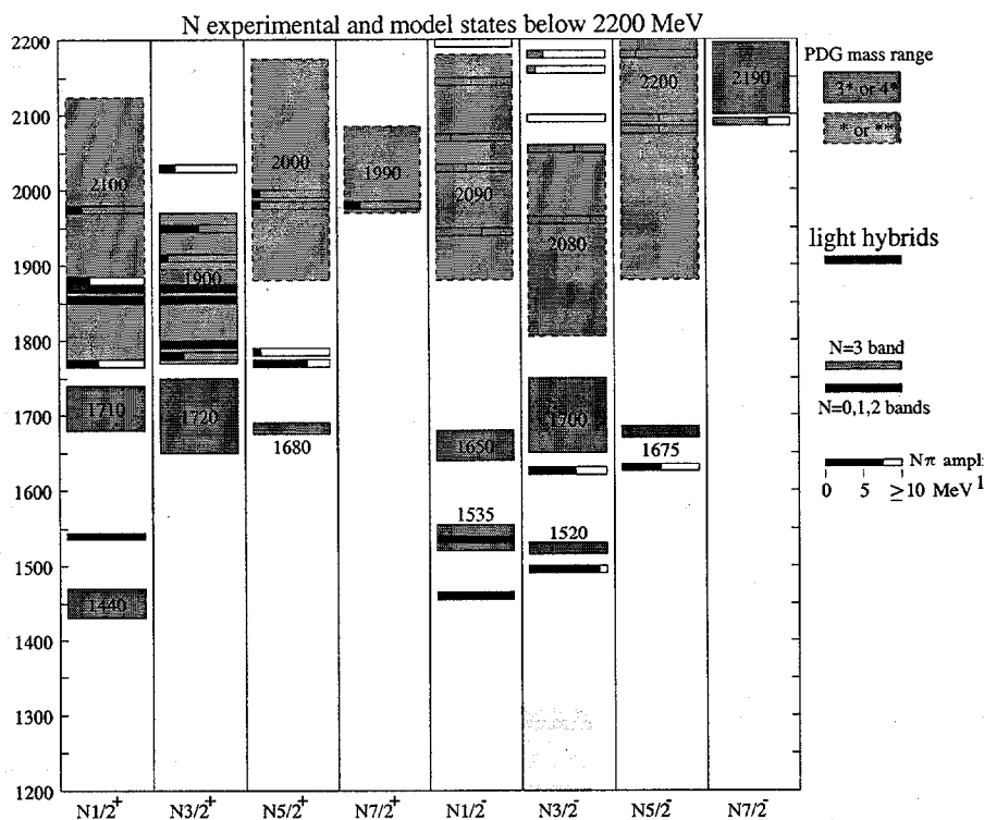
Figure 2: The four light N flavor hybrid baryons found by Capstick and Page [13] in the flux-tube model, compared to experiment. The estimated error is \pm 100 MeV (light blue background).
