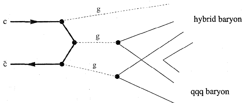
Figure 4: Production of qqqg states from J/\Psi radiative decays occurs at O(\alpha_s^5) (followed by nonperturbative pair production), which leads J/\Psi \rightarrow ggg \rightarrow (qqq) + (\bar{q}q\bar{q}) by one power of \alpha_s .
